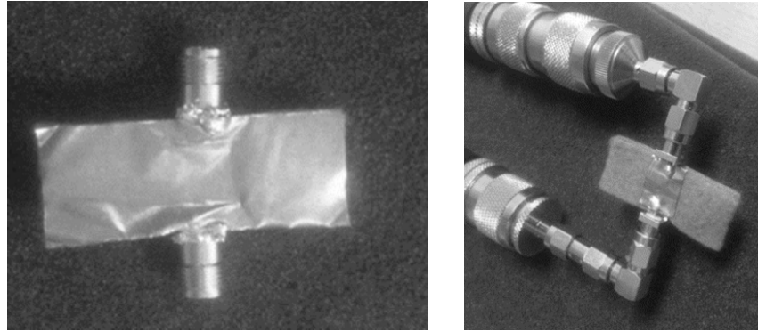
Figure 4.5 Photographs of the set up for loss tangent measurement.
