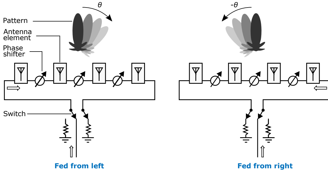
Figure 2.4 Principle of a bidirectional series-fed phased array.
