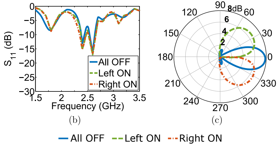
Figure 5.21 (a) Top view of a uniform EBG, (b) |S_{11}| Vs. frequency, and (c) azimuth plane ( xy ) pattern.
